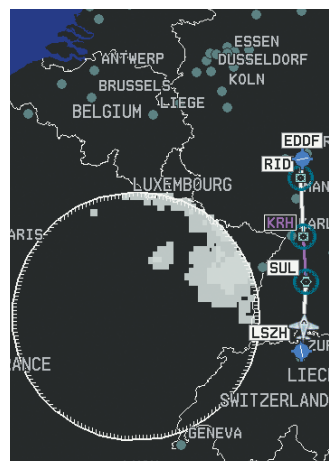
Figure 10-27 Off-Route Data Request
