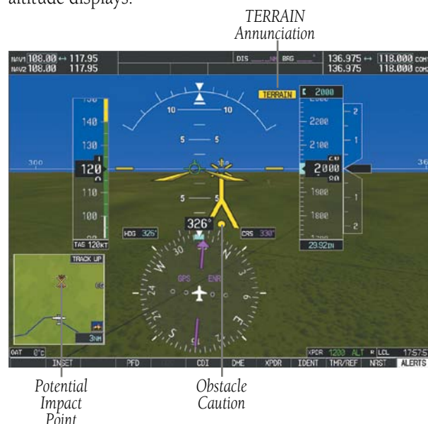
Figure 11-10 Obstacle
