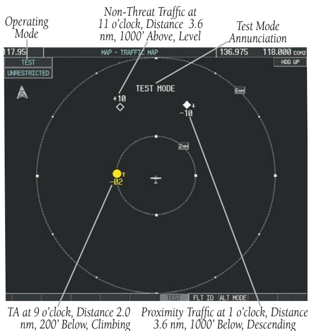
Figure 10-31 Test Mode
