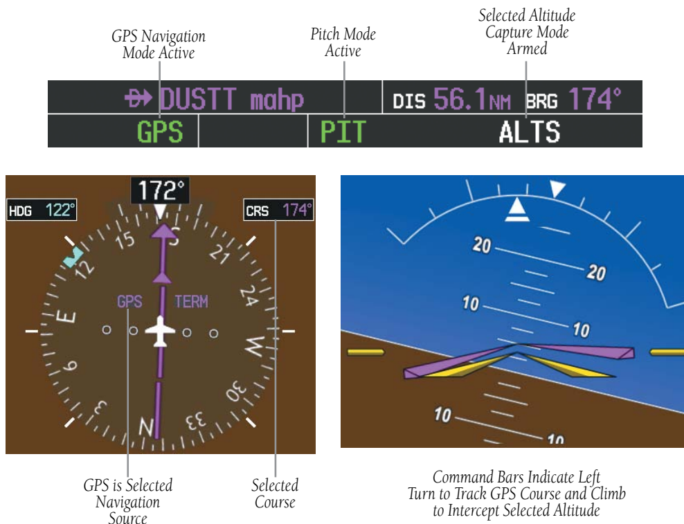
Figure 6-22 Navigation Mode
