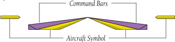
Figure 6-2 Command Bars
