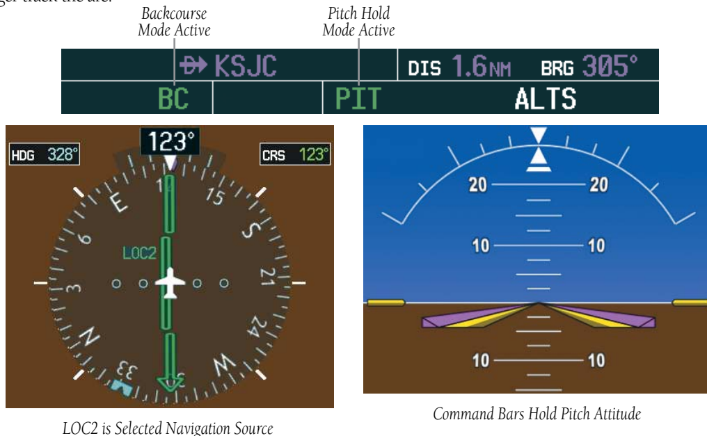
Figure 6-25 Backcourse Mode
