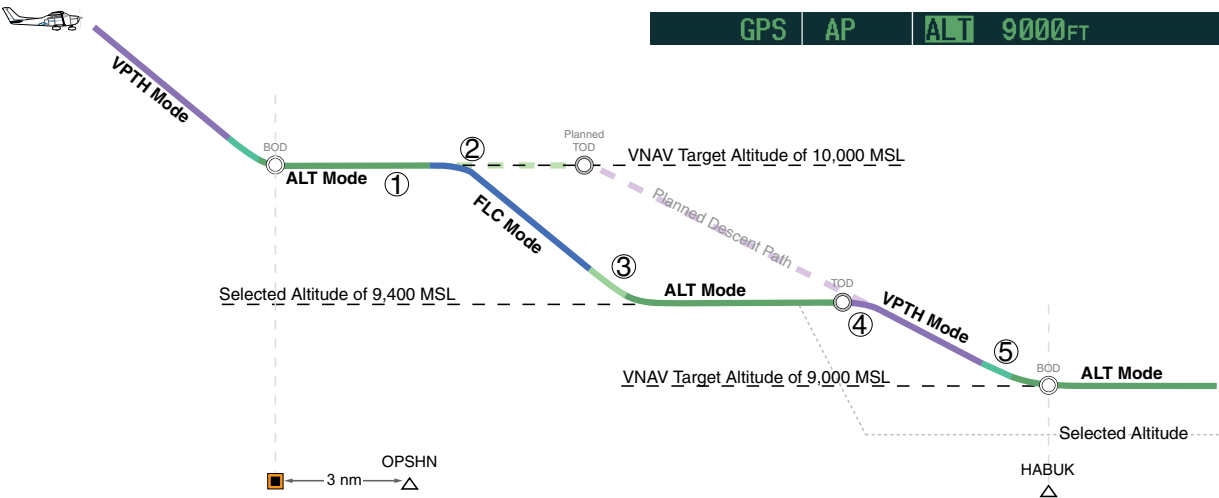
Figure 6-36 Non-path Descent
