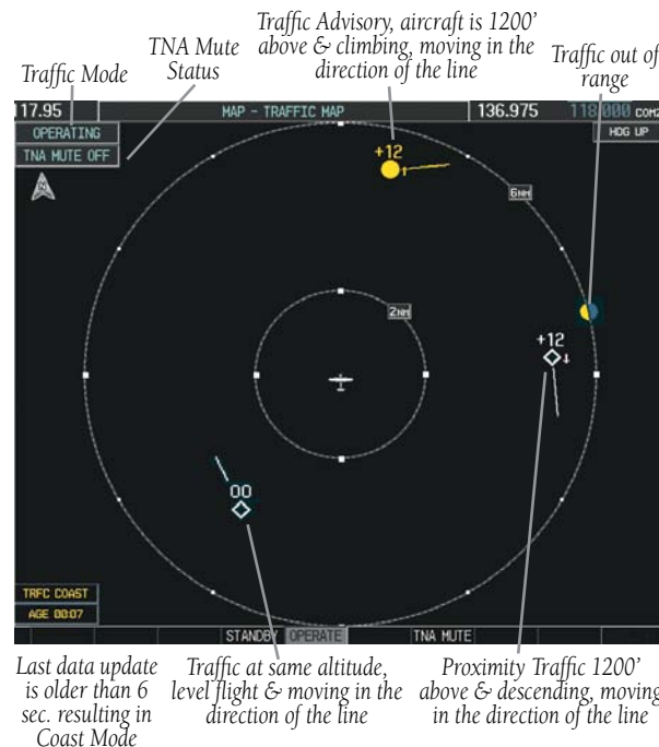
Figure 10-30 Traffic Map Page
