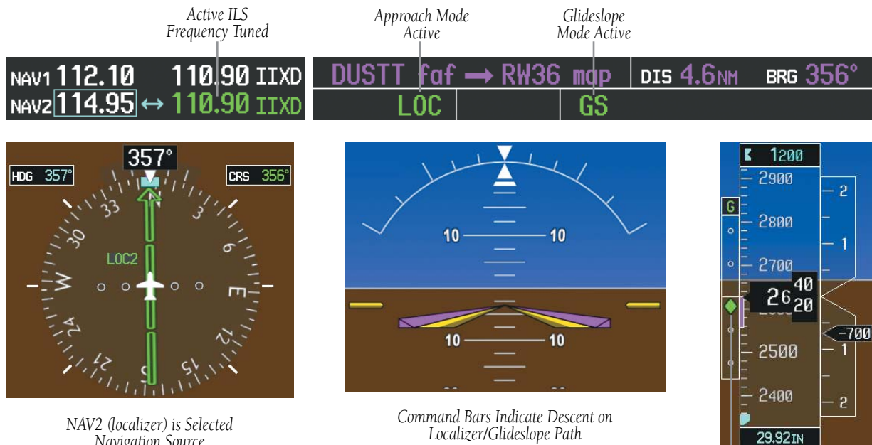
Figure 6-17 Glide Slope Mode
