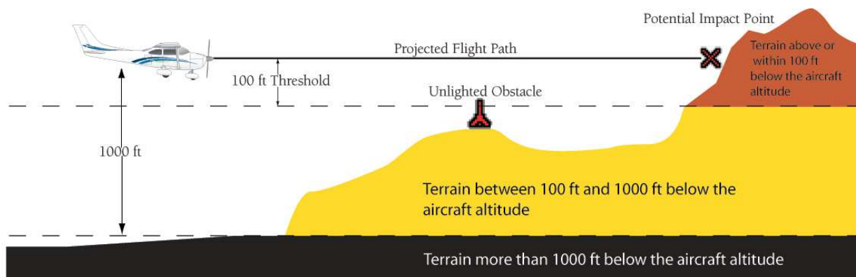
Figure 10-46 Terrain-Color Code
