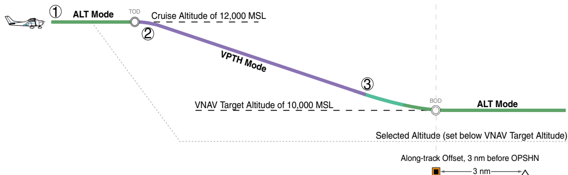
Figure 6-35 VPTH Descent
