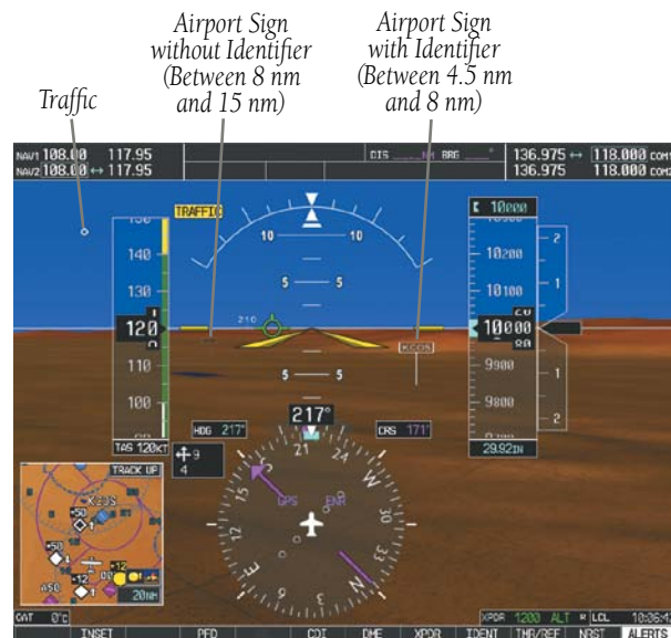
Figure 11-7 Airport Signs
