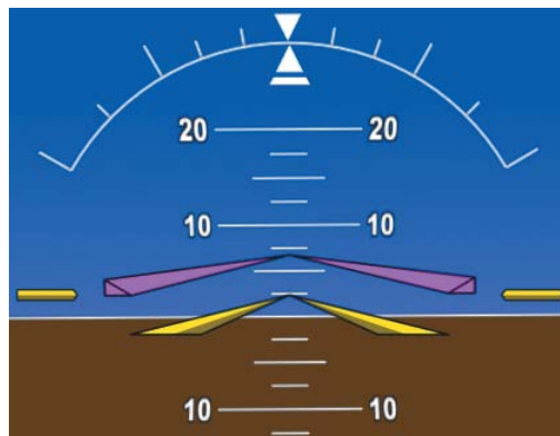
Figure 6-19 Go Around Mode
