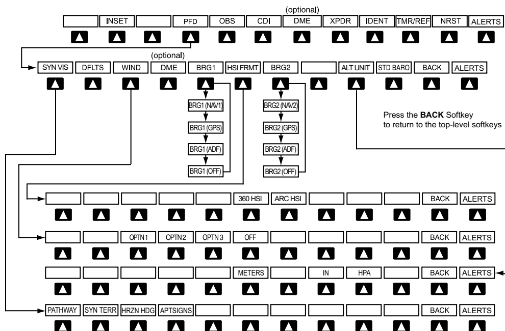
Figure 1-3 PFD Configuration Softkeys
