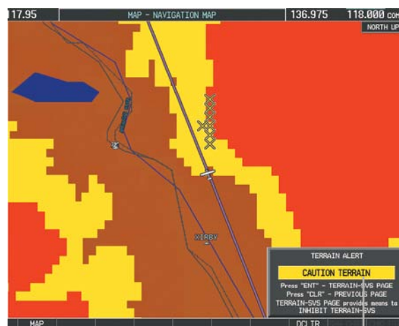
Figure 10-43 TERRAIN-SVS Alert Annunciations
