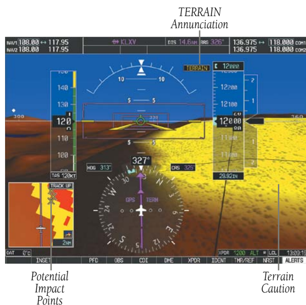
Figure 11-9 Terrain Alert
