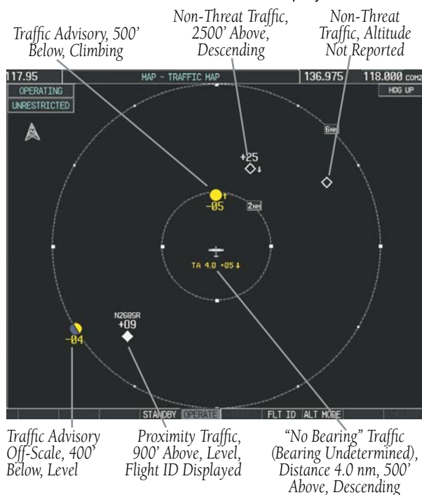
Figure 10-32 Traffic Map
