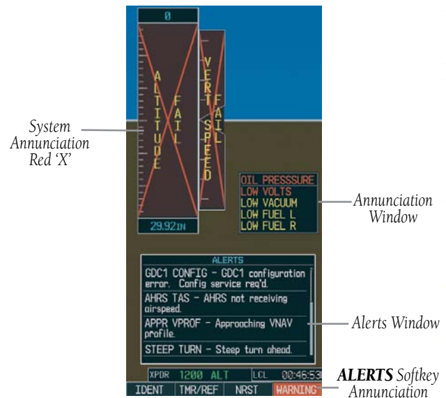
Figure 13-1 G1000 Alerting System
