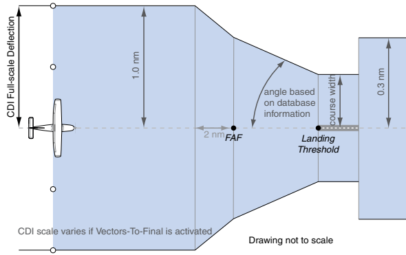
Figure 2-24 Typical LNAV/VNAV and LPV Approach CDI Scaling (SBAS Systems Only)
