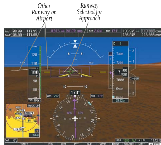
Figure 11-8 Airport Runways
